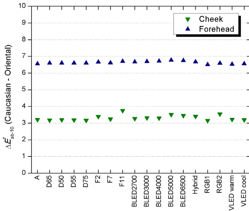
Figure 7 CIELAB colour differences between Caucasian and Oriental women’s faces, considering separately the results for forehead and cheek, under 18 illuminants.
