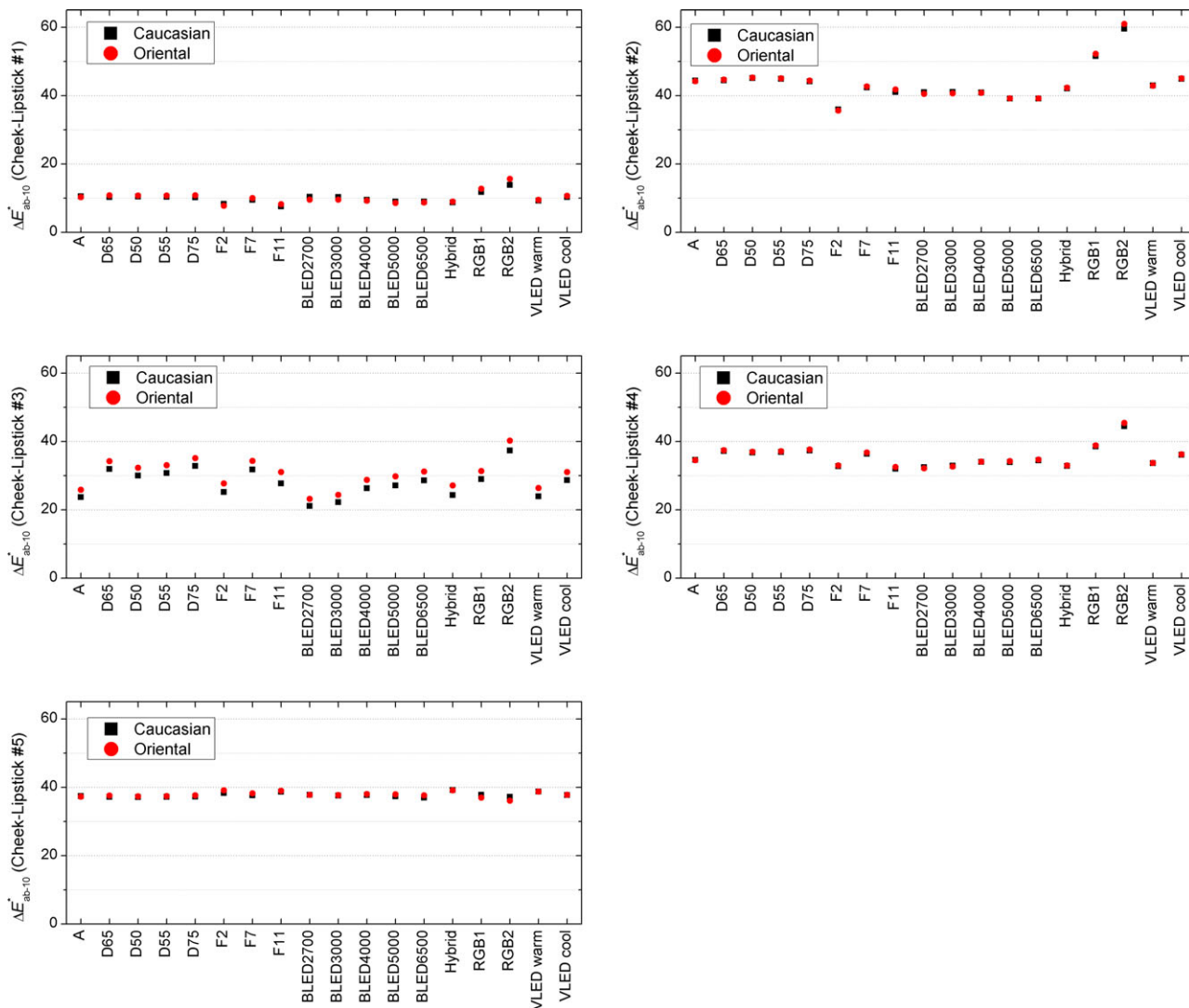
Figure 9 CIELAB colour differences between each of the five lipsticks and the cheek in Caucasian and Oriental women, under 18 illuminants.
