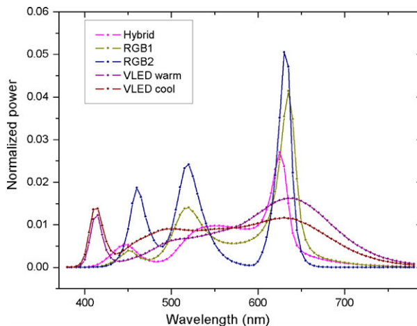
Figure 2 Representative SPDs of five white LEDs using three different technologies (hybrid, RGB and phosphor-converted violet) [22].
