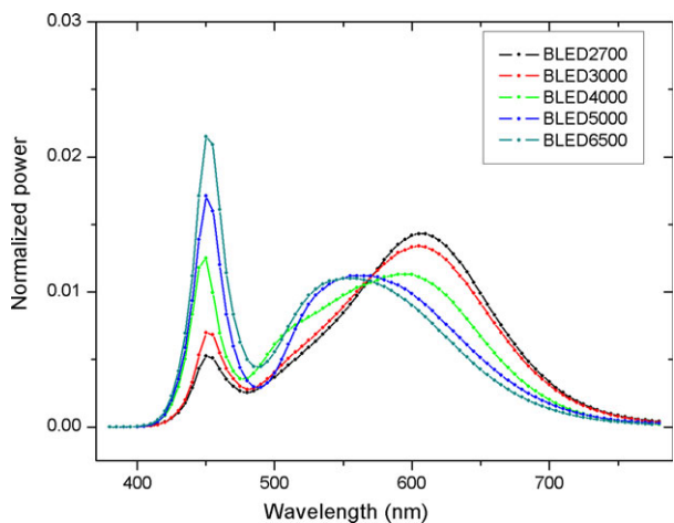
Figure 1 Representative SPDs of five phosphor-converted blue LEDs (BLEDs), with CCTs from approximately 2700 K to 6500 K [22].
